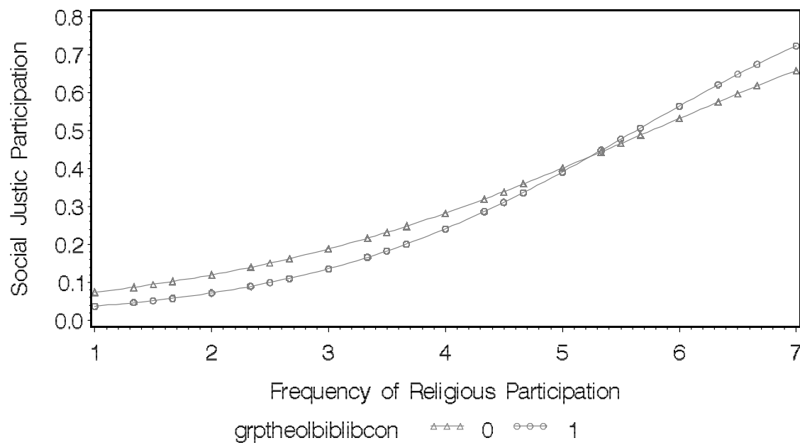
Online Figure 10.3. Example follow up logistic regression plot for SJ participation. Triangles = people in liberal congregations. Circles = people in conservative congregations.
