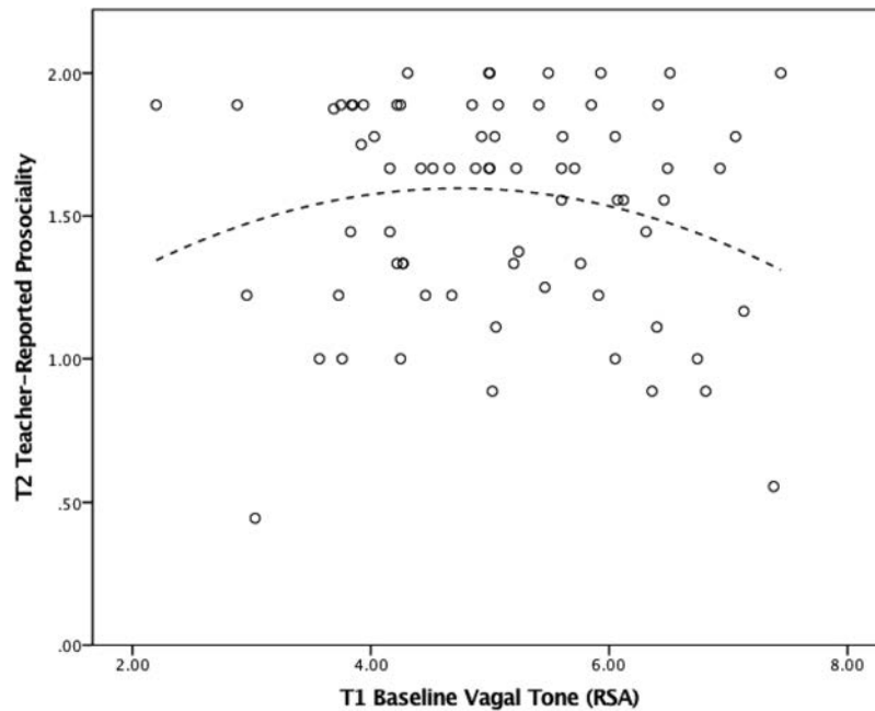
Figure 6. Quadratic line fit to data to represent relation between baseline respiratory sinus arrhythmia (RSA) at preschool age and children's teacher-reported prosociality 5.5 years later in Study 3.
