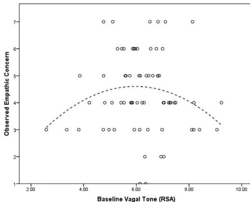
Figure 2. Quadratic line fit to data to represent relation between baseline respiratory sinus arrhythmia (RSA) and children's observed empathic concern in Study 2.
