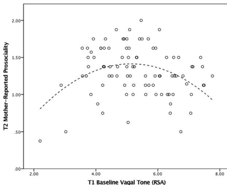
Figure 5. Quadratic line fit to data to represent relation between baseline respiratory sinus arrhythmia (RSA) at preschool age and children's mother-reported prosociality 5.5 years later in Study 3.
