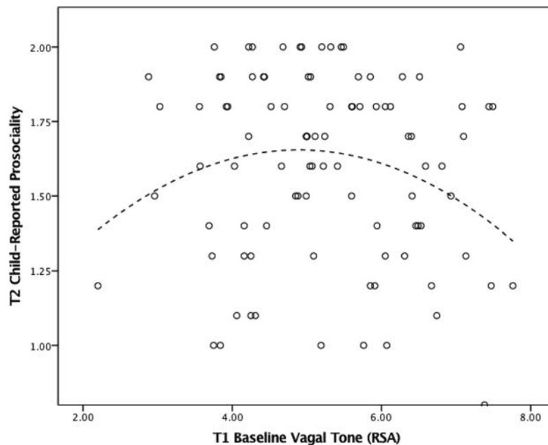
Figure 4. Quadratic line fit to data to represent relation between baseline respiratory sinus arrhythmia (RSA) at preschool age and children's self-reported prosociality 5.5 years later in Study 3.
