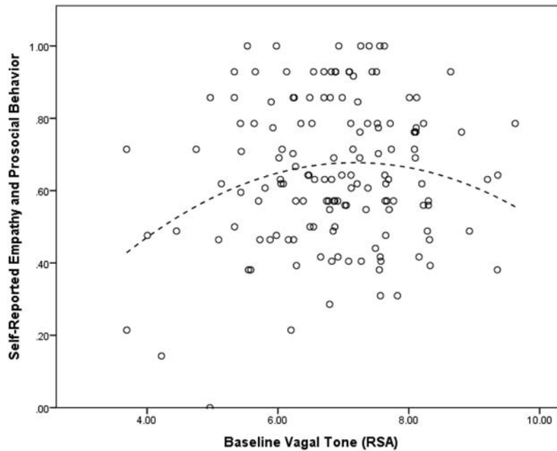
Figure 1. Quadratic line fit to data to represent relation between baseline respiratory sinus arrhythmia (RSA) and children's self-reported prosociality in Study 1.
